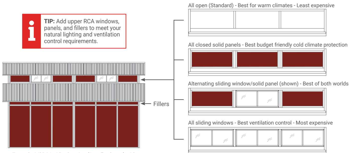
Example 24' RCA side elevation (2 stalls shown) with alternating RCA windows/panels and upper fillers.
