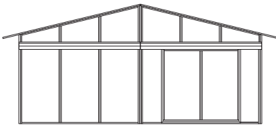
24' Gable End Hay/Storage Room Elevation (Shown with 8' Sliding Door Half Open)
