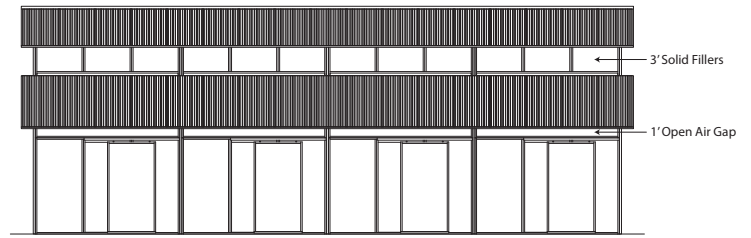
48' Shedrow Side Elevation (Shown with Doors Half Open)
