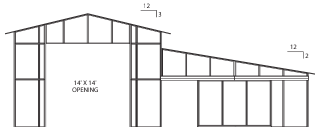
24' Gable/24' Shedrow Barn (12' Breezeway) Elevation (Shown with 12' Sliding Doors Half Open)
