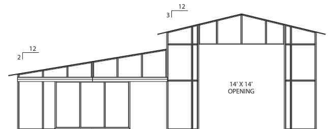
24' Gable/24' Shedrow Barn (12' Breezeway) Elevation (Shown with 12' Sliding Doors Half Open)
