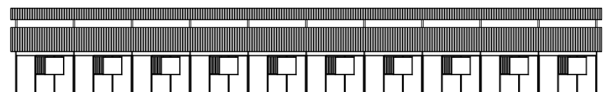
Side Elevation (Shown with Grill Window and Shutters Half Open)
