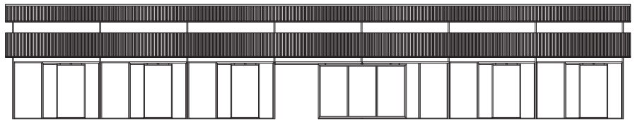
Side Elevation Showing 12' Side Breezeway Door Half Open (Shown with 4' Rear Doors Half Open)
