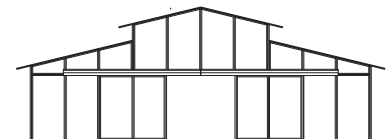
16' Breezeway Raised Center Aisle (RCA) Barn Elevation (Shown with 8' Sliding Doors Half Open)
