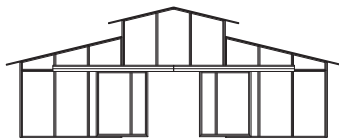
12' Breezeway Raised Center Aisle (RCA) Barn Elevation (Shown with 6' Sliding Doors Half Open)
