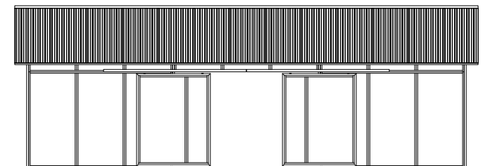
Front View Elevation (Shown with 6' Doors Half Open)
