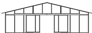
12' Breezeway Gable Barn Elevation (Shown with 6' Sliding Doors Half Open)
