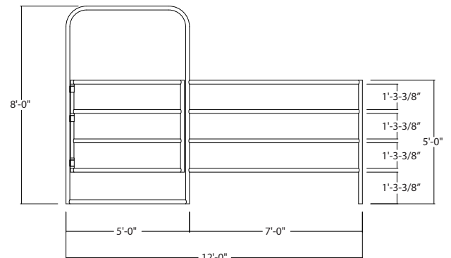
Standard 4-Rail Gate Panel
