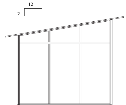
Single Slope Side View Elevation
