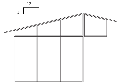
Side View Elevation (Showing Cantilever Overhang)
